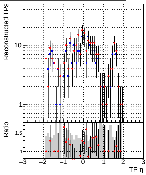
Legend: DQM_mkFit_TT_base_noSel (blue squares), DQM_mkFit_TT_retrainOldFiles_v2_8iter_noSel (red diamonds)
