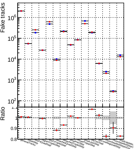
Number —●— DQM_mkFit_TT_retrainOldFiles_v2_8iter_noSel
