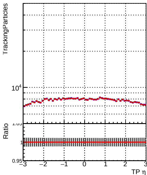
—•— DQM_mkFit_TT_base_noSel —•— DQM_mkFit_TT_retrainOldFiles_v2.8iter_noSel
