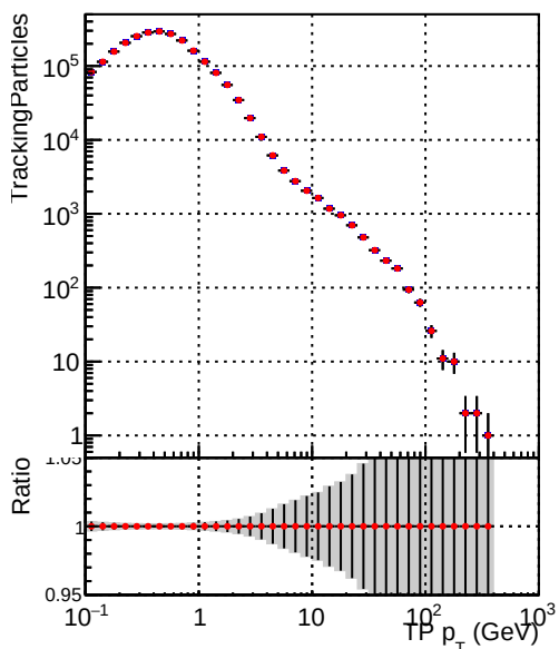
—•— DQM_mkFit_TT_base_noSel —•— DQM_mkFit_TT_retrainOldFiles_v2.8iter_noSel
