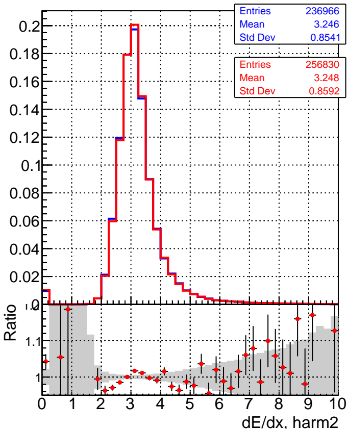
—■ DQM_mkFit_TT_base_noSel —● DQM_mkFit_TT_retrainOldFiles_v2_8iter_noSel
