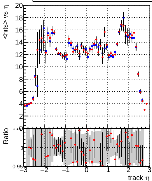
Legend: — DQM_mkFit_TT_base_noSel — DQM_mkFit_TT_retrainOldFiles_v2_8iter_noSel mean hit
