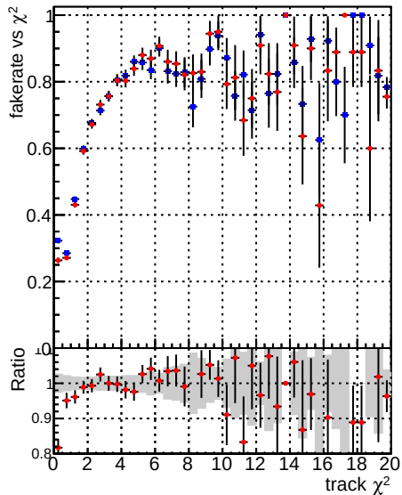
Fake rate vs. \chi^2 Legend: —●— DQM mkFit TT base_noSel —×— DQM mkFit TT retrainOldFiles_v2 8iter_noSel
