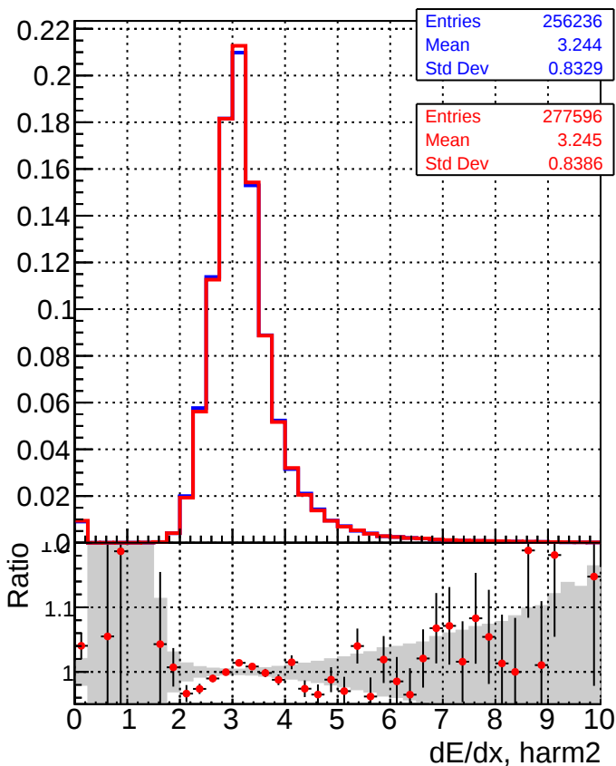
— DQM_mkFit_TT_base_noSel — DQM_mkFit_TT_retrainOldFiles_v2_8iter_noSel
