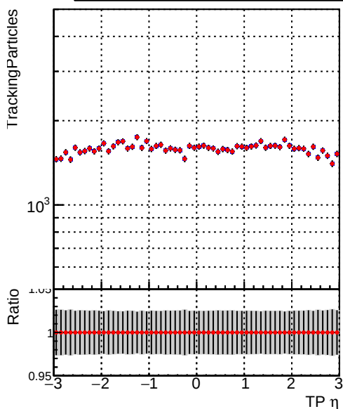
N of simulated tracks vs TP \eta Legend: —•— DQM_mkFit_TT_base_noSel —•— DQM_mkFit_TT_retrainOldFiles_v2_8iter2_noSel
