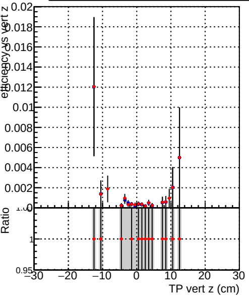
Efficiency vs TP vert z (cm) Legend: DQM_mkFit_TT_base_noSel DQM_mkFit_TT_retrainOldFiles_v2_8iter2_noSel
