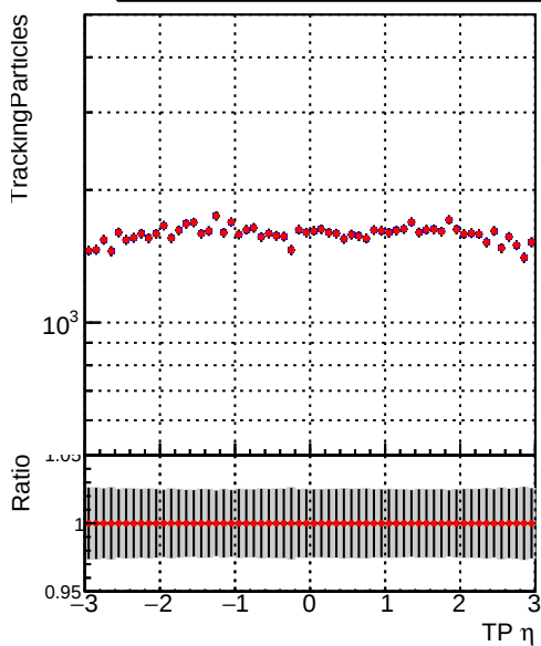
N of simulated tracks vs \eta Legend: DQM_mkFit_TT_base_noSel (blue dots), DQM_mkFit_TT_retrainOldFiles_v2_8iter2_noSel (red dots)
