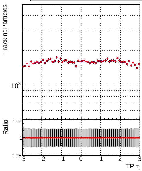
Legend: DQM_mkFit_TT_base_noSel (blue circles), DQM_mkFit_TT_retrainOldFiles_v2_8iter2_noSel (red circles)
