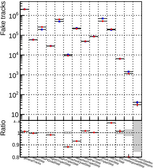
Number —●— DQM_mkFit_TT_retrainOldFiles_v2_8iter2_noSel
