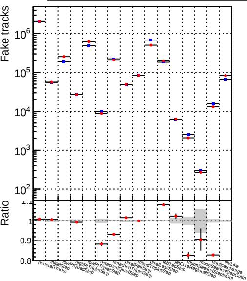
Number —●— DQM_mkFit_TT_retrainOldFiles_v2_8iter2_noSel
