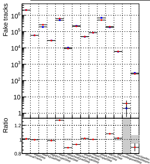
Number 1 DQM_mkFit_TT_retrainOldFiles_v2_8iter2_noSel
