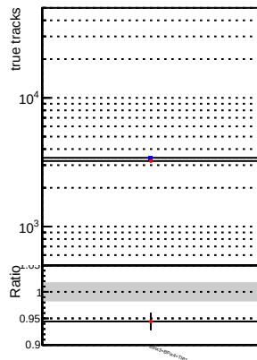
N of reco track vs. \chi^2 —•— DQM_mkFit_TT_base_noSel —•— DQM_mkFit_TT_retrainOldFiles_v2_8iter2_noSel
