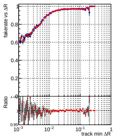
Legend: DQM_mkFit_TT_base_noSel (blue line with dots), DQM_mkFit_TT_retrainOldFiles_v2_8iter2_noSel (red line with dots)
