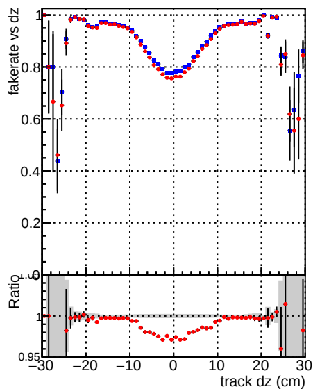
Fake rate vs dz —●— DQM_mkFit_TT_base_noSel —●— DQM_mkFit_TT_retrainOldFiles_v2_8iter2_noSel
