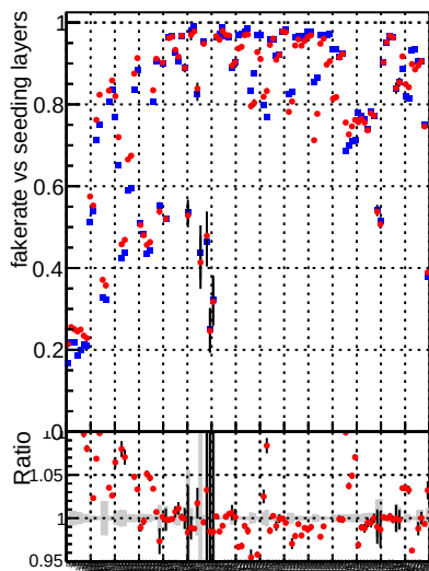
Fake rate vs. —■— DQM mkFit TT base_noSel —■— DQM mkFit TT retrainOldFiles_v2 8iter2_noSel
