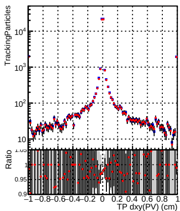
N of sim DQM_mkFit_TT_base_noSel DQM_mkFit_TT_retrainOldFiles_v2_8iter2_noSel
