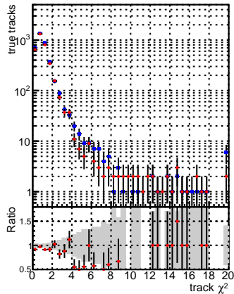
Legend: DQM_mkFit_TT_base_noSel DQM_mkFit_TT_retrainOldFiles_v2_8iter2_noSel
