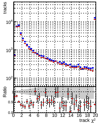
N of reco track vs. \chi^2 for DQM mkFit TT_base_noSel and DQM mkFit TT_retrainOldFiles_v2_8iter2_noSel
