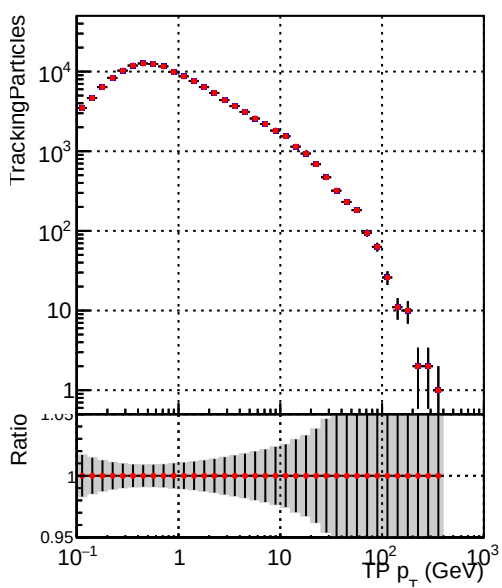
—•— DQM_mkFit_TT_base_noSel —•— DQM_mkFit_TT_retrainOldFiles_v2.8iter2_noSel
