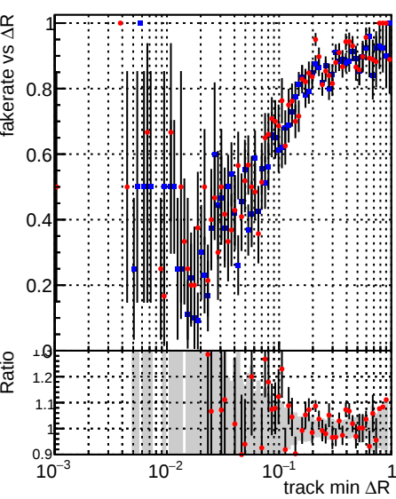
Legend: DQM_mkFit_TT_base_noSel (blue squares), DQM_mkFit_TT_retrainOldFiles_v2_8iter2_noSel (red circles)
