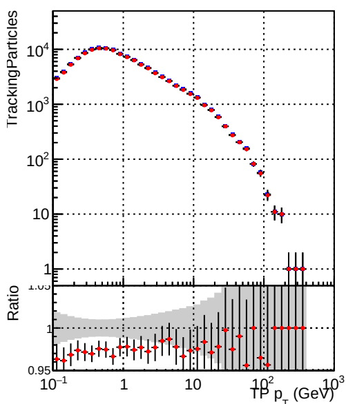
Legend: DQM_mkFit_TT_base_noSel (blue squares), DQM_mkFit_TT_retrainOldFiles_v2_8iter2_noSel (red circles)
