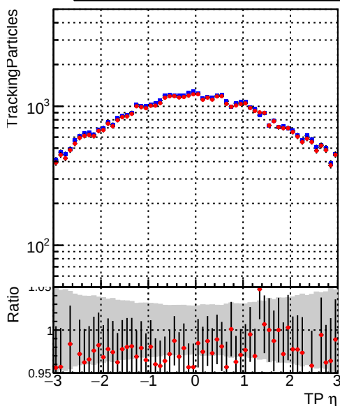
Legend: DQM_mkFit_TT_base_noSel (blue squares), DQM_mkFit_TT_retrainOldFiles_v2_8iter2_noSel (red circles)
