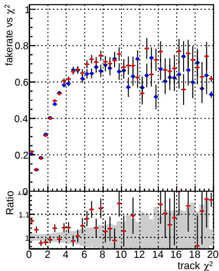
Fake rate vs. \chi^2 Legend: DQM_mkFit_TT_base_noSel (blue diamonds) DQM_mkFit_TT_retrainOldFiles_v2_8iter2_noSel (red diamonds)
