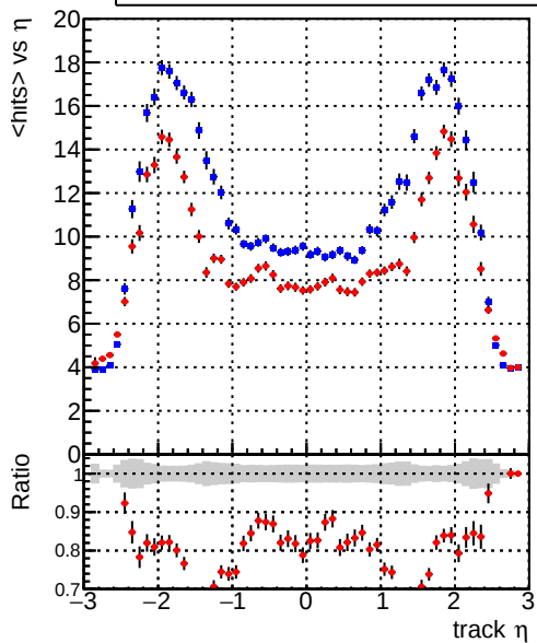
mean hit — DQM_mkFit_TT_base_noSel — DQM_mkFit_TT_retrainOldFiles_v2_8iter2_noSel
