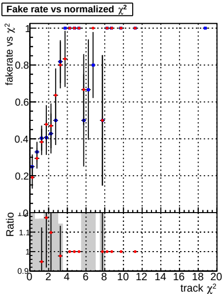
Fake rate vs. —●— DQM_mkFit_TT_base_noSel —●— DQM_mkFit_TT_retrainOldFiles_v2_8iter2_noSel
