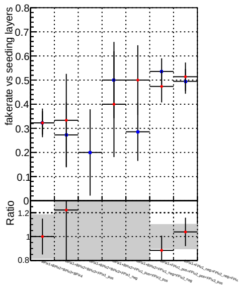
Fake rate vs. —●— DQM_mkFit_TT_base_noSel —●— DQM_mkFit_TT_retrainOldFiles_v2_8iter2_noSel
