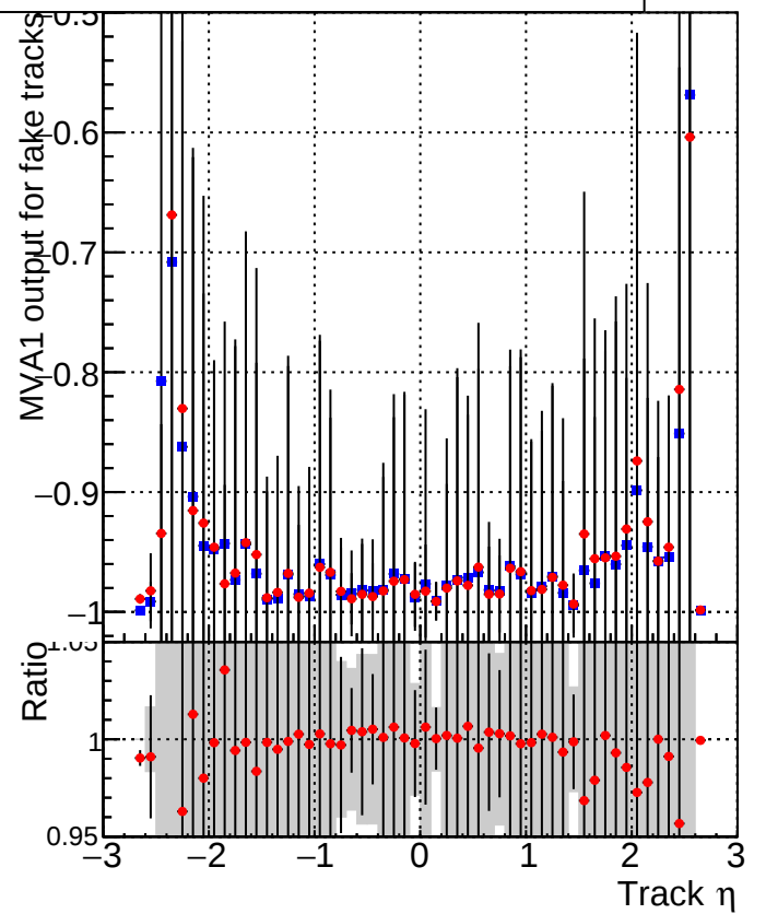
MVA1 of associated tracks (recoToSim) vs. track \eta Legend: DQM_mkFit_TT_base_noSel (blue squares) DQM_mkFit_TT_retrainOldFiles_v2_8iter2_noSel (red diamonds)
