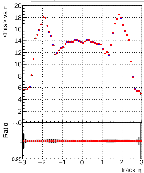
mean hits vs \eta Legend: DQM_mkFit_TT_base_noSel (blue line), DQM_mkFit_TT_retrainOldFiles_v2_8iter2_noSel (red line)
