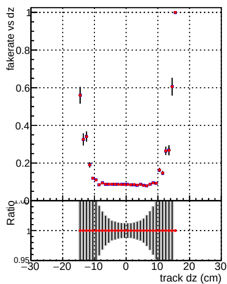
Fake rate vs dz — DQM_mkFit_TT_base_noSel — DQM_mkFit_TT_retrainOldFiles_v2_8iter2_noSel
