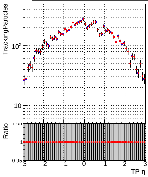
Legend: DQM_mkFit_TT_base_noSel (blue diamonds), DQM_mkFit_TT_retrainOldFiles_v2_8iter2_noSel (red diamonds)
