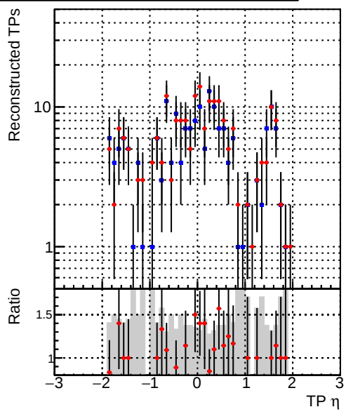
Legend: DQM_mkFit_TT_base_noSel (blue diamonds), DQM_mkFit_TT_retrainOldFiles_v2_8iter2_noSel (red diamonds)
