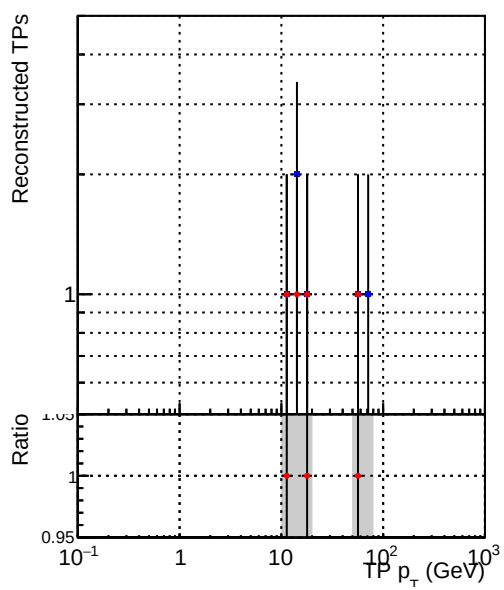
Legend: - \bullet DQM_mkFit_TT_base_noSel - \bullet DQM_mkFit_TT_retrainOldFiles_v2_8iter2_noSel
