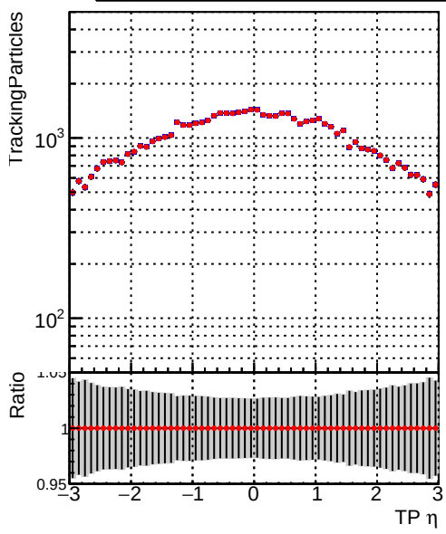
Legend: - \bullet DQM_mkFit_TT_base_noSel - \bullet DQM_mkFit_TT_retrainOldFiles_v2_8iter2_noSel
