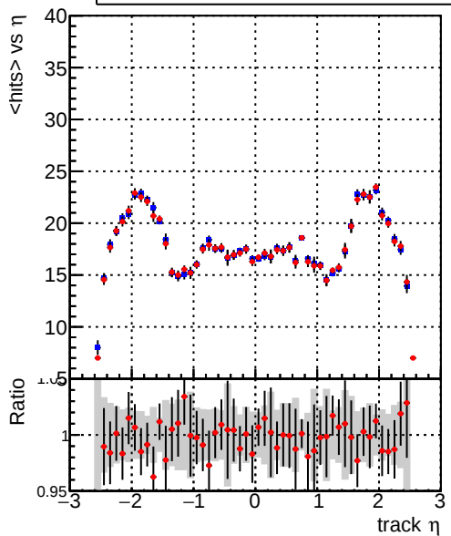
mean hit — DQM_mkFit_TT_base_noSel — DQM_mkFit_TT_retrainOldFiles_v2_8iter2_noSel
