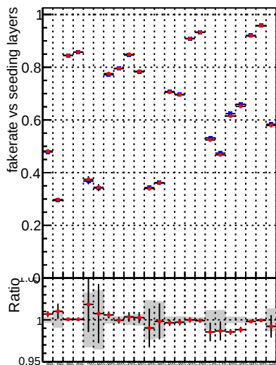
Fake rate vs. —•— DQM_mkFit_TT_base_noSel —•— DQM_mkFit_TT_retrainOldFiles_v2_noSel
