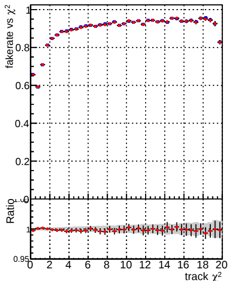
Fake rate vs. —•— DQM_mkFit_TT_base_noSel —•— DQM_mkFit_TT_retrainOldFiles_v2_noSel
