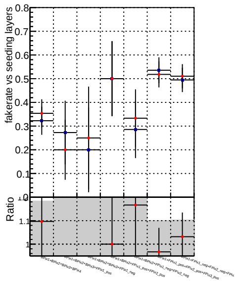
Fake rate vs. — DQM_mkFit_TT_base_noSel — DQM_mkFit_TT_retrainOldFiles_v2_noSel
