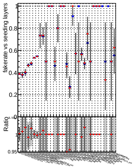
Fake rate vs. —•— DQM_mkFit_TT_base_noSel —•— DQM_mkFit_TT_retrainOldFiles_v2_noSel
