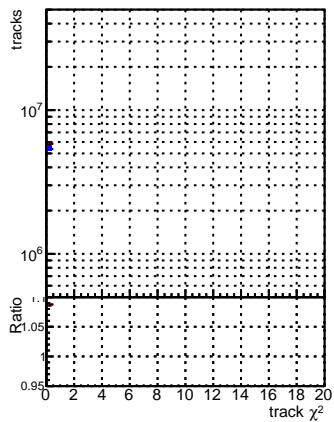
N of reco track vs. \chi^2 base after noSel ok DQM mkFit RetrainV2 after noSel ok
