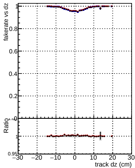
DOM mkFit TT baseR3 noSel ok DOM mkFit TT base 3iter noSel ok DOM mkFit TT RetrainV2 3iter noSel ok
