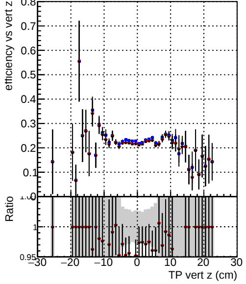
Efficiency vs. sim PV z —●— DQM_mkFit_TT_baseR3_noSel_ok —●— DQM_mkFit_TT_base_8iter_noSel_ok —●— DQM_mkFit_TT_Retrainv2_8iter_noSel_ok
