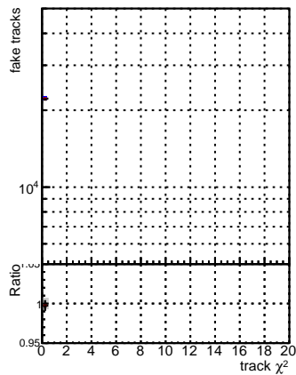
N of associated (recoToSim) fake tracks vs. \chi^2 for different selection criteria
