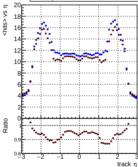
— DQM_mkFit_TT_baseR3_noSel_ok — DQM_mkFit_TT_base_8iter_noSel_ok — DQM_mkFit_TT_Retrainv2_8iter_noSel_ok mean hit
