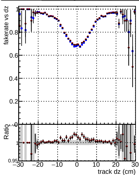
DOM mkFit TT baseR3 noSel ok DOM mkFit TT base 8iter noSel ok DOM mkFit TT RetrainV2 8iter noSel ok
