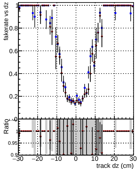
DOM mkFit TT baseR3 noSel ok DOM mkFit TT baseR3 noSel ok DOM mkFit TT baseR3 noSel ok DOM mkFit TT baseR3 noSel ok DOM mkFit TT baseR3 noSel ok DOM mkFit TT baseR3 noSel ok
