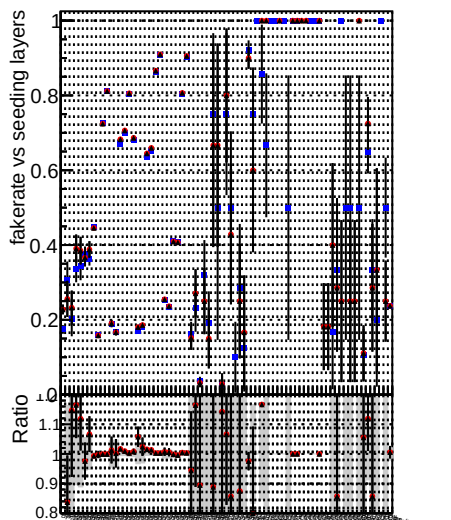
Fake rate vs. DOM mkFit TT baseR3 noSel ok DOM mkFit TT base 8iter noSel ok DOM mkFit TT Retrainv2 8iter noSel ok
