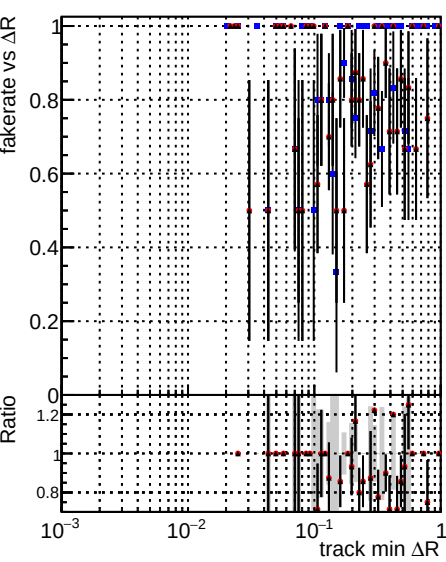
Fake rate vs \Delta R (track, jet) DQM mkFit TT baseR3 noSel_ok DQM mkFit TT base 8iter noSel_ok DQM mkFit TT Retrainv2 8iter noSel_ok
