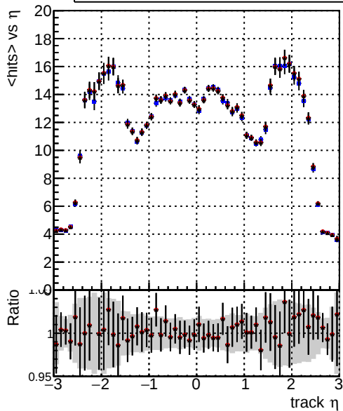
mean hit — DQM_mkFit_TT_baseR3_noSel_ok — DQM_mkFit_TT_base_8iter_noSel_ok — DQM_mkFit_TT_Retrainv2_8iter_noSel_ok
