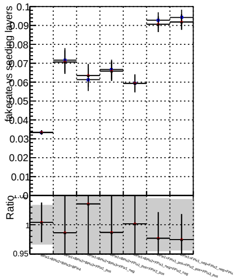
Fake rate vs. — DOM mkFit TT baseR3 noSel ok — DOM mkFit TT base 8iter noSel ok — DOM mkFit RetrainV2 8iter noSel ok
