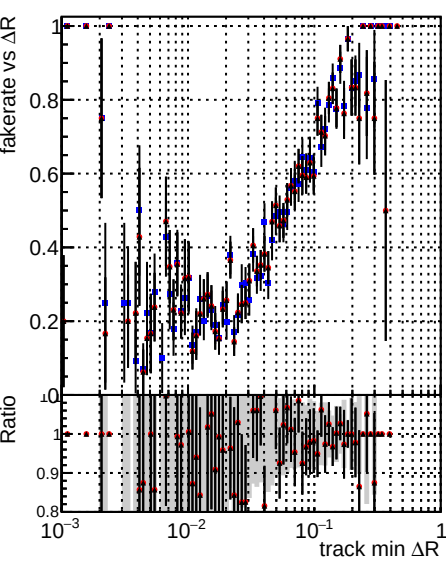
Legend: DQM_mkFit_TT_baseR3_noSel_ok (blue), DQM_mkFit_TT_base_8iter_noSel_ok (red), DQM_mkFit_TT_Retrainv2_8iter_noSel_ok (black)
