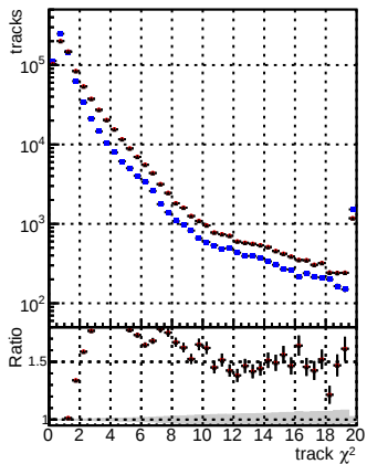
N of reco track vs. s DQM mkFit TT base. 8iter noSel ok DQM mkFit TT Retrainv2 8iter noSel ok
